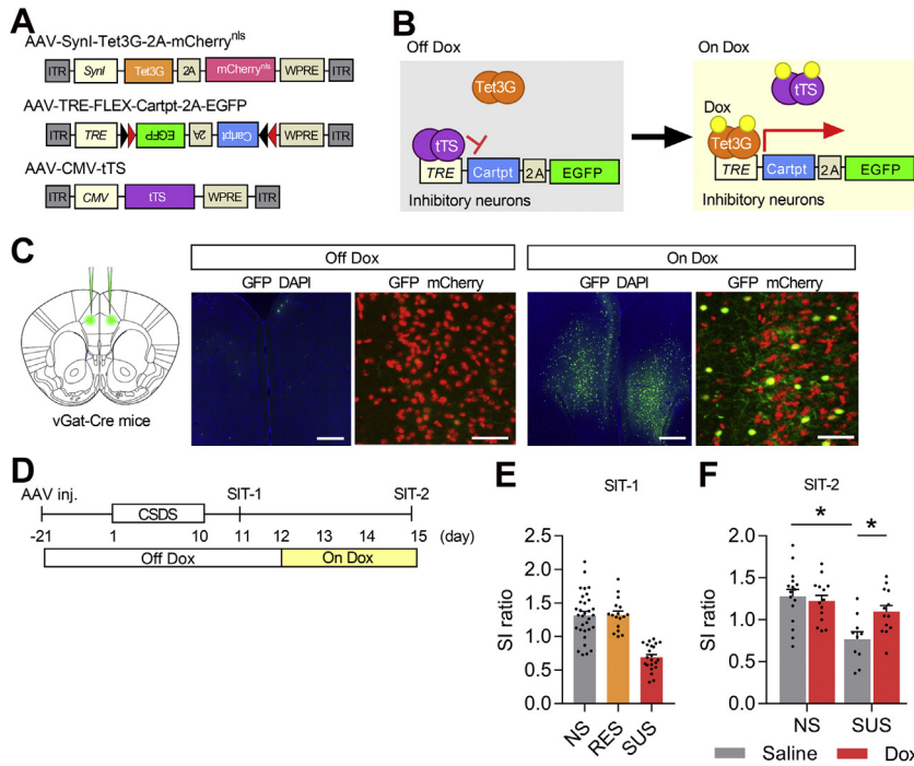
Figure 6. CART peptides in GABAergic neurons of the aCC have an antidepressant effect in stress-susceptible mice. (A) AAV-mediated spatiotemporal gene expression strategy using a cocktail of AAV-Syn1-Tet3G-2A-mCherry nlis , AAV-TRE-FLEX-Cartpt-2A-EGFP, and AAV-CMV-tTS. (B) Schematic representation of dox- and Cre-dependent regulation of TRE-mediated gene expression in the inhibitory neurons using both the tetracycline-dependent activator (Tet3G) and repressor (tTS). Without dox, tTS represses TRE-mediated gene expression, whereas in the presence of dox, Tet3G activates TRE-mediated gene expression specifically in Cre-expressing cells. (C) AAV microinjection into the aCC region of vGat-Cre mice. Region-specific and dox-regulated expression of mCherry in the aCC is shown. Scale bar = 500 μm for low-magnification images (GFP and DAPI) and 50 μm for high-magnification images (GFP and mCherry). (D) Experimental timeline of Cartpt induction in inhibitory neurons of the aCC after the termination of CSDD episodes. Mice injected with a cocktail of AAVs were subjected to 10-day CSDD and were tested by SIT-1, followed by the administration of dox for 3 days (twice per day). Mice were tested using a SIT-2. (E) SI ratio after CSDD exposure (SIT-1). The CSDD group was divided into two groups (RES and SUS groups) based on their SI ratios. n = 32 for NS and 39 for CSDD (both RES and SUS). (F) SI ratio before (SIT-1) and after (SIT-2) dox admin-
