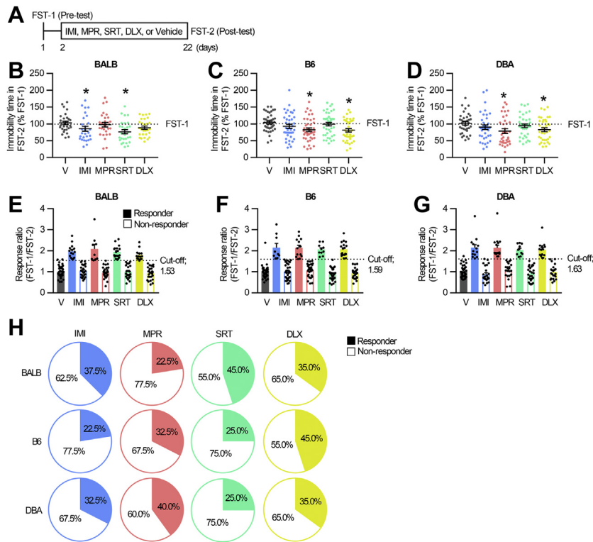
Figure 1. Identification of subgroups of responders and nonresponders to antidepressant treatments in inbred strains of mice. (A) Experimental design. Mice were tested using the FST-1 before a 3-week treatment with either tap water (V), IMI, MPR, SRT, or DLX. After long-term treatment with the antidepressant, a second FST (FST-2) was performed. (B–D) Immobility time in the FST-2 (% FST-1) in BALB/c (BALB) (B) , C57BL/6J (B6) (C) , and DBA/2 (DBA) (D) mice. n = 36–40 in each group. *p < .05 vs. FST-1 in the corresponding treatment. (E–G) Response ratio (immobility time in FST-1/immobility time in FST-2). The responder and nonresponder subgroups were identified by the mean + 2 SD method with a cutoff value. n = 36–40 in each group. (H) Distribution of responders and nonresponders in each strain of mice treated with specific antidepressants. n = 36–40 in each group. All data are presented as mean \pm SEM. DLX, duloxetine; FST, forced swim test; IMI, imipramine; MPR, maprotiline; SRT, sertraline; V, vehicle.
