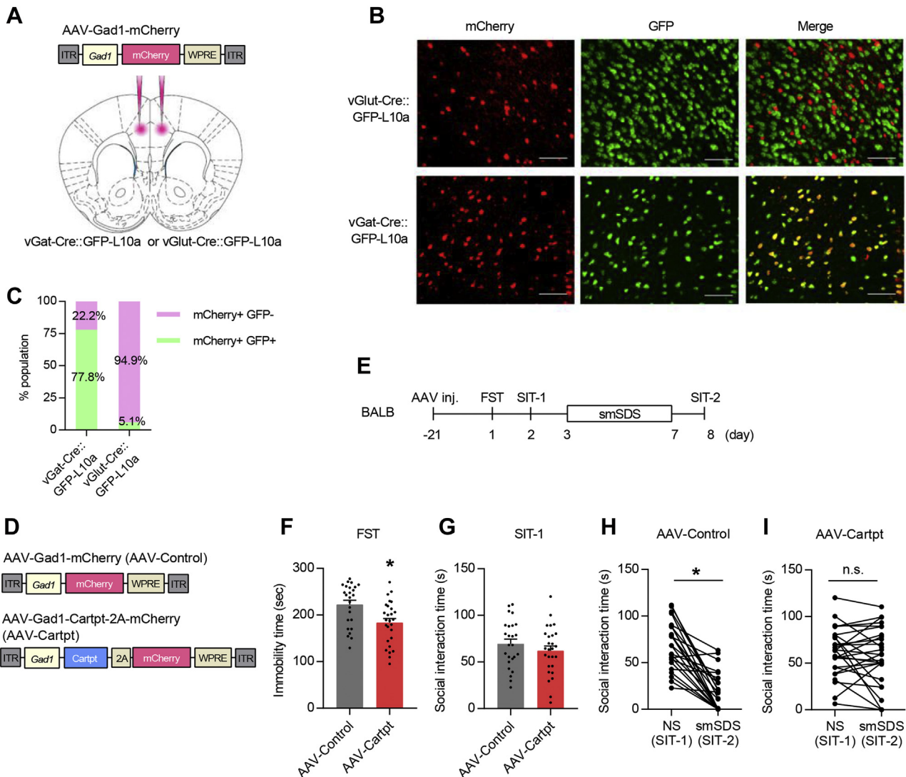
Figure 5. AAV-mediated CART peptide overexpression in aCC GABAergic neurons drives antidepressant-like behaviors and stress resilience in stress-vulnerable strains. (A) AAV vectors used for mCherry overexpression under the control of the Gad1 promoter (AAV-Gad1-mCherry). To validate the cell-type specificity of the Gad1 promoter in these AAVs, AAV-Gad1-mCherry was injected bilaterally into the aCC region of either vGat-Cre::GFP-L10a mice or vGlut-Cre::GFP-L10a mice (as reporter mice). (B) Fluorescence signals of EGFP (green) and mCherry (red) in the aCC of vGat-Cre::GFP-L10a mice (top panels) and vGlut-Cre::GFP-L10a mice (bottom panels). Colocalization of EGFP and mCherry is seen in vGat-Cre::GFP-L10a, but not in vGlut-Cre::GFP-L10a mice. Scale bar = 100 \mu m. (C) Quantification of the percentage of mCherry-positive cells (red) in the aCC region that overlap with GFP-positive cells (green). mCherry expression driven by the Gad1 promoter is enriched in GFP-positive cells of vGat-Cre::GFP-L10a mice, but not of vGlut-Cre::GFP-L10a mice. n = 4 in each group; 425–685 mCherry-positive cells per group were analyzed. (D) AAV vectors used for mCherry (AAV-control) and Cartpt (AAV-Cartpt) overexpression under the control of the Gad1 promoter. (E) Experimental paradigm used for behavioral testing. (F) Mice injected with AAV-Cartpt show reduced immobility time compared with mice injected with AAV-control in the FST. n = 25 –27 in each group. * p < .05 . (G) Mice injected with AAV-Cartpt show a comparable SI time to that of mice injected with AAV-control in nonstressed conditions. n = 25 –27 in each group. * p < .05 . (H, I) The SI time of stressed mice injected with AAV-control was significantly lower than that of nonstressed mice injected with AAV-control (H) , whereas this reduction was prevented in mice injected with AAV-Cartpt (I) . n = 12 –16 in each group. * p < .05 . All data are presented as mean \pm SEM. AAV, adeno-associated virus; aCC, anterior cingulate cortex; EGFP, enhanced green fluorescent protein; FST, forced swim test; GABAergic, gamma-aminobutyric acidergic; inj., injection; NS, nonstress control; n.s., not significant; SIT, social interaction test; smSDS, subchronic and mild social defeat stress.
