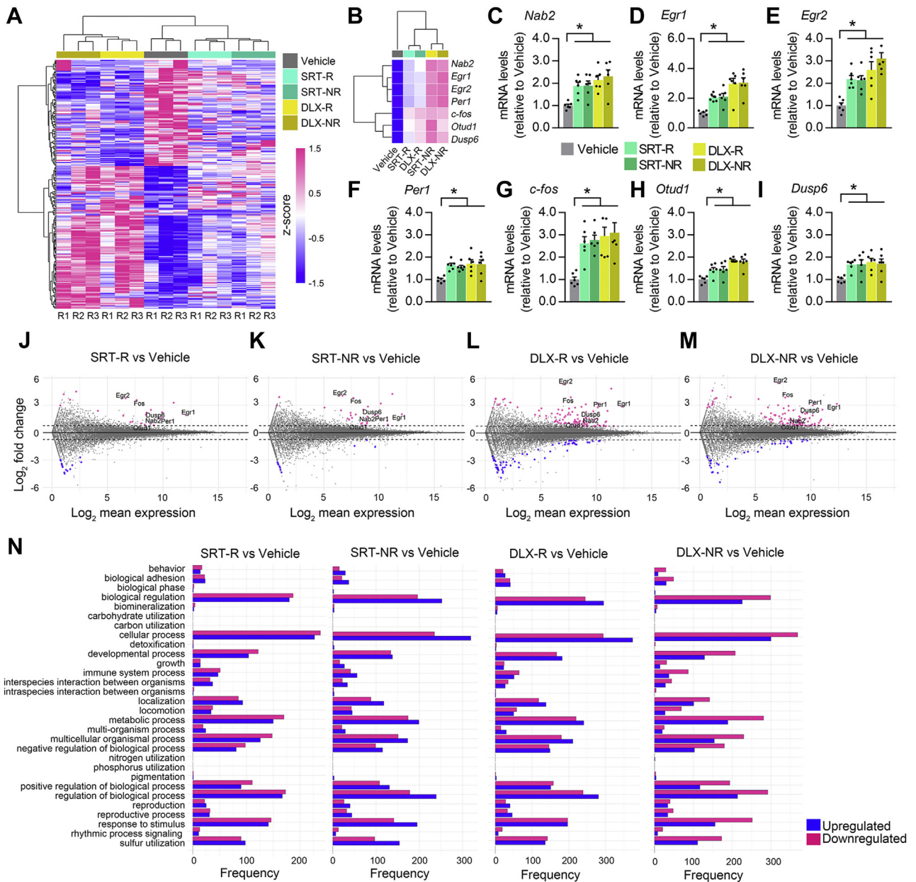
Figure 2. RNA sequencing reveals transcriptional alterations in the medial prefrontal cortex of antidepressant responders and nonresponders. (A) Heatmap representation of differentially expressed genes (fold change >1.3 and false discovery rate p < .1 ) in the responder and nonresponder groups to treatment with SRT and DLX (three replicates per group). (B) Heatmap representation of differentially expressed genes (fold change >1.3 and false discovery rate p < .1 ) that were commonly upregulated in both responders and nonresponders to treatment with SRT and DLX. (C–I) Real-time polymerase chain reaction validation of the alterations in gene expression identified in the differentially expressed gene analysis presented in (B) . n = 6 in each group. *Adjusted p < .05 vs. the vehicle. (J–M) MA plot of the results of the differential expression analysis in SRT-R (J) , SRT-NR (K) , DLX-R (L) , or DLX-NR (M) . (N) Gene Ontology profile analysis (biological process) of differentially expressed genes ( p < .05 ) between the vehicle and SRT-R, SRT-NR, DLX-R, or DLX-NR (red, upregulated genes; blue, downregulated genes). The x-axis displays the number of differentially expressed genes, and the y-axis indicates the Gene Ontology terms. All data are presented as mean \pm SEM. DLX-NR, DLX nonresponders; DLX-R, duloxetine responders; mRNA, messenger RNA; SRT-NR, sertraline nonresponders; SRT-R, sertraline responders.
