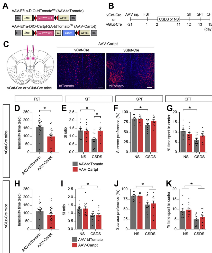
Figure 4. CART peptides in GABAergic neurons of the aCC drive antidepressant-like behaviors and stress resilience. (A) AAV vectors used for the control construct (AAV-tdTomato) and Cartpt overexpression (AAV-Cartpt). (B) Experimental paradigm of behavioral testing. (C) AAV microinjection into the aCC. Region-specific expression of tdTomato in the aCC is shown. Scale bar = 100 \mu m. (D–G) Effects of Cartpt overexpression in GABAergic neurons of the aCC on the FST (D) , SIT (E) , SPT (F) , and OFT (G) . n = 23–24 for FST and n = 11–13 for SIT, SPT, and OFT in each group. *p < .05 . (H–K) Effects of Cartpt overexpression in glutamatergic neurons of the aCC on the FST (H) , SIT (I) , SPT (J) , and OFT (K) . n = 23–24 for the FST and n = 11–14 for the SIT, SPT, and OFT in each group. *p < .05 . All data are presented as mean \pm SEM. AAV, adeno-associated virus; aCC, anterior cingulate cortex; CSDS, chronic social defeat stress; FST, forced swim test; GABAergic, gamma-aminobutyric acidergic; inj, injection; NS, nonstress control; OFT, open field test; SIT, social interaction test; SPT, sucrose preference test.
