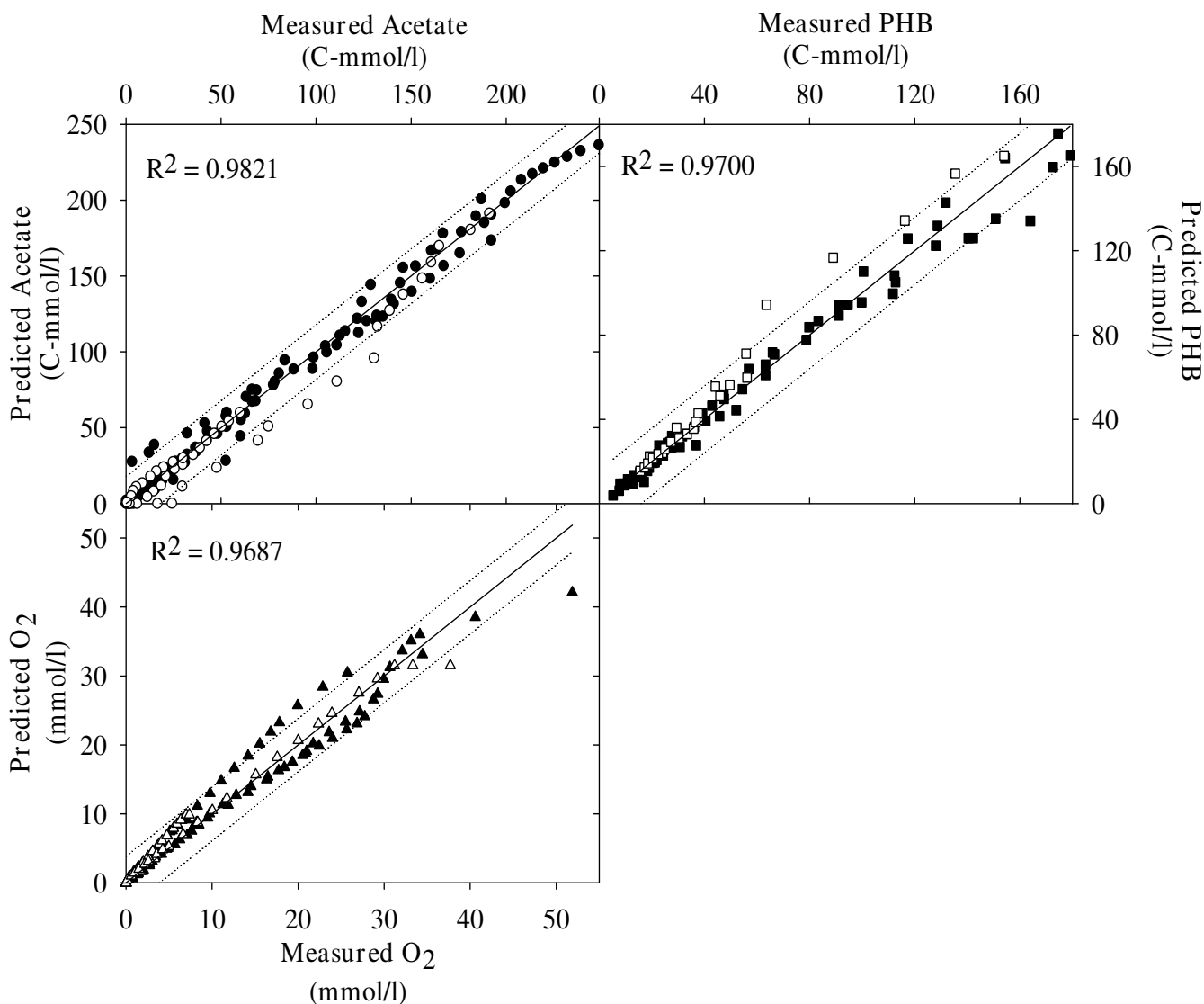
Figure 2 Modelling results. Figure shows the results obtained for acetate enriched cultures under acetate feeding conditions. Full symbols represent parameter estimation results and open symbols the model validation results. Dashed lines are the 95% confidence limits for the parameter estimation and model validation results.
