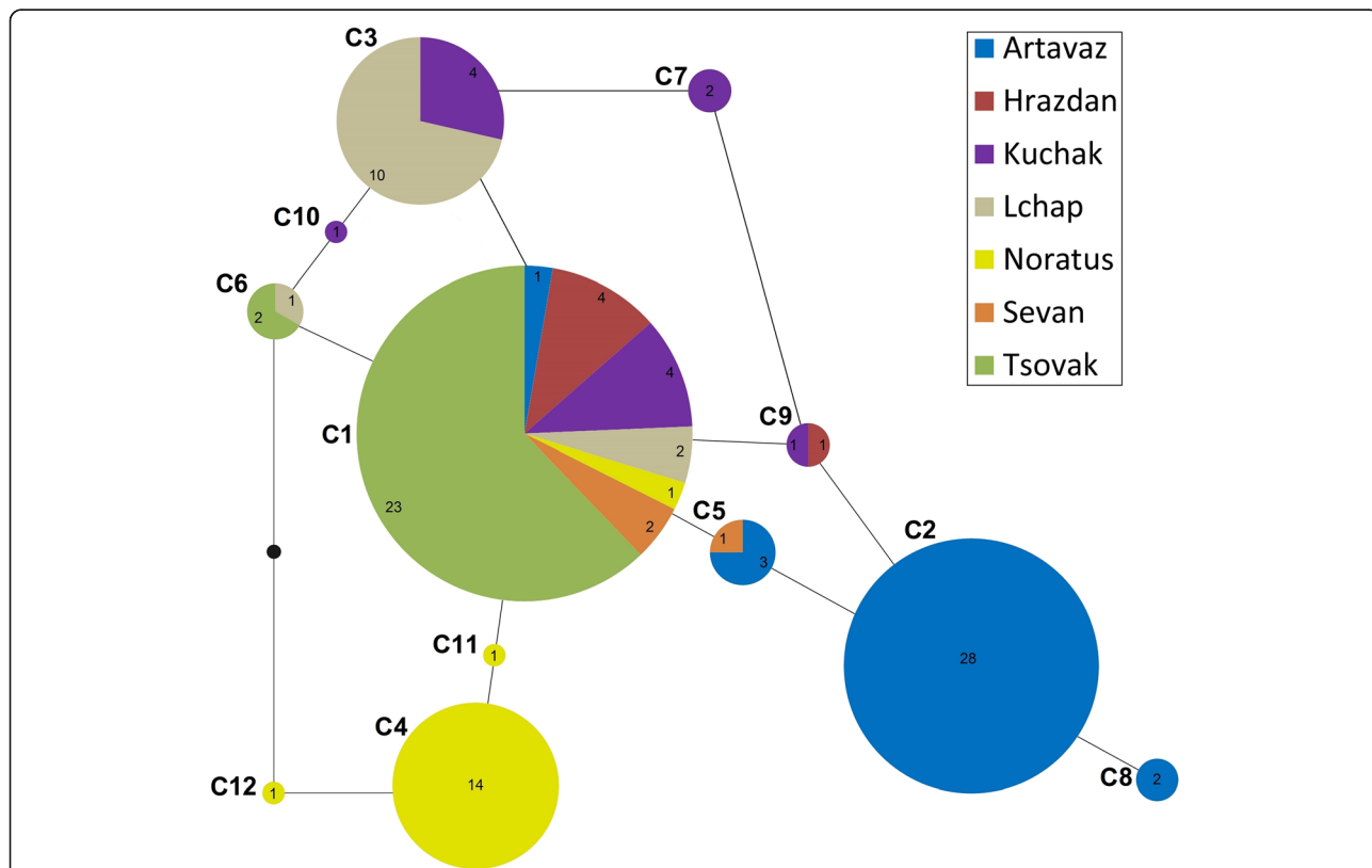
Fig. 2 A statistical parsimony (TCS) network showing the geographic associations of the 12 clones in parthenogenetic Darevskia unisexualis . Analyses used differences in the number of repeats, but not indels. Number of individuals in populations given in pie slices
