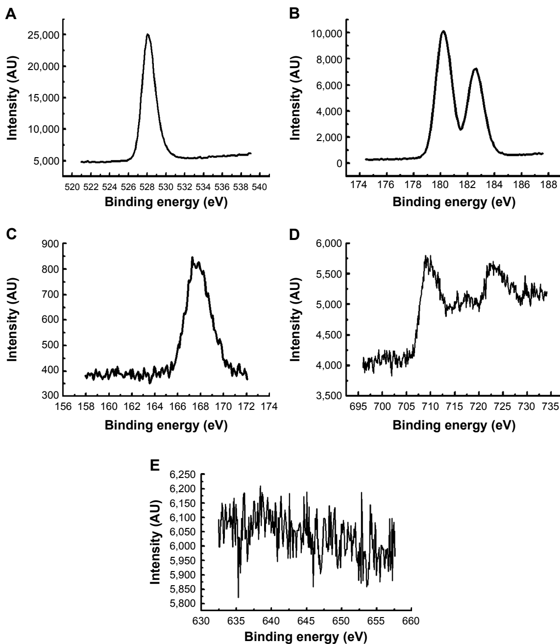
Figure 1 X-ray photoelectron spectra of iron(+3)–manganese-promoted sulfated zirconia. Notes: (A) O^{2-} (1s); (B) Zr^{4+} (3d5/2); (C) Fe^{3+} (S 2p); (D) for Fe(111) (2p3/2, 2p1/2); and (E) Mn^{4+} (2p3/2, 2p1/2).
