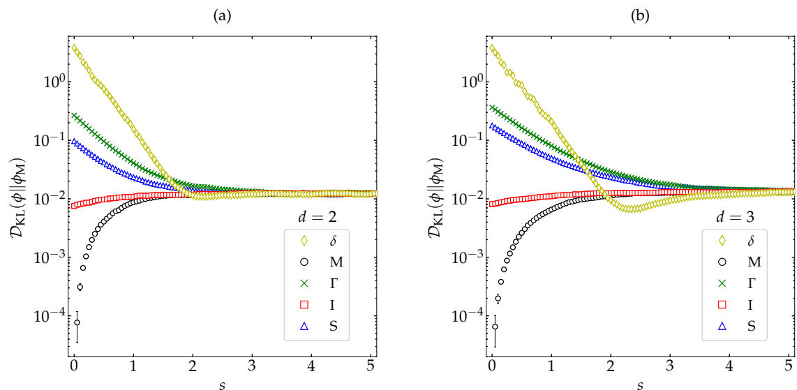
Figure 7. Evolution of \mathcal{D}_{\text{KL}}(\phi||\phi_M) (in logarithmic scale) for a coefficient of restitution \alpha = 0.1 as a function of the average number of collisions per particle for hard (a) disks and (b) spheres. Symbols represent MD simulation results. Five different initial conditions are considered (see Appendix B): \delta ( \diamond ), M ( \circ ), \Gamma ( \times ), I ( \square ), and S ( \triangle ). The error bars are smaller than the size of the symbols, except when \mathcal{D}_{\text{KL}}(\phi||\phi_M) \lesssim 10^{-4} for the initial condition M.
