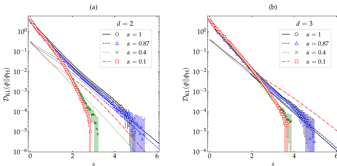
Figure 8. Evolution of \mathcal{D}_{\text{KL}}(\phi \parallel \phi_{\text{H}}) (in logarithmic scale) as a function of the average number of collisions per particle for (a) disks and (b) spheres. Symbols represent MD simulation results, while the lines correspond to the theoretical prediction (40) (the thin dashed lines for the first stage of the evolution meaning that it was necessary to take the real part). The values of the coefficient of restitution are \alpha = 0.1 ( \square ), 0.4 ( \times ), 0.87 ( \triangle ), and 1 ( \circ ). The error bars in the simulation data are smaller than the size of the symbols, except when \mathcal{D}_{\text{KL}}(\phi \parallel \phi_{\text{M}}) \lesssim 10^{-4} .
