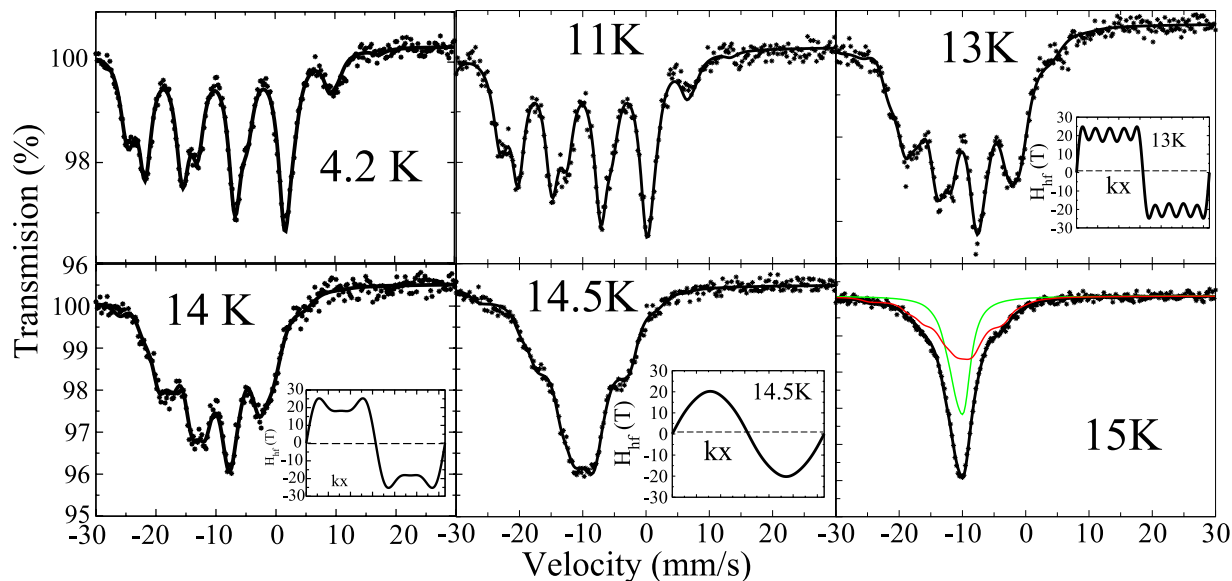
Figure 5. ^{151}\text{Eu} Mössbauer spectra in \text{EuIrAl}_4\text{Si}_2 between 4.2 K and 15 K (see text). The modulations at 13 K, 14 K and 14.5 K along the propagation vector k are shown next to the corresponding spectrum.
