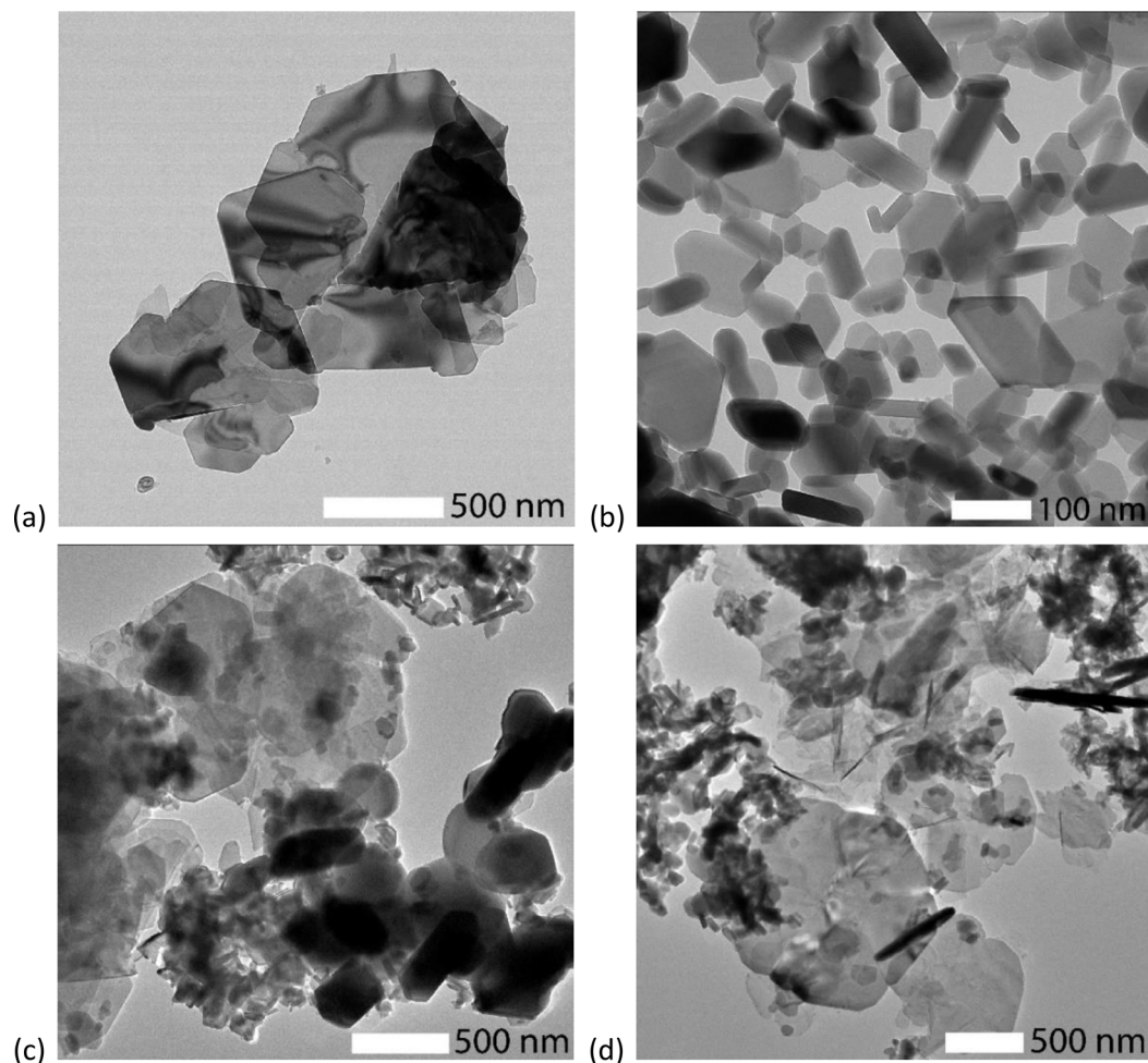
Fig. 3 TEM images of (a) AC100 shows large platelet shaped crystallites \text{SrFe}_{12}\text{O}_{19} from the autoclave synthesis (b) SSM100 shows regular shaped free-standing crystallites of \text{SrFe}_{12}\text{O}_{19} , (c) DM50, and (d) WM50 gives an overview of the two mixtures, where both thin platelets and smaller thick crystallites can be observed.
