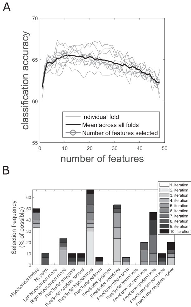
Fig. 2. Result of sequential forward feature selection (SFS). (A) Performance as a function of number of selected features. The thin gray lines correspond to each of the 10 training sets in the ADNI+AIBL 10FCV dataset, and the thick black line is the average performance across the 10 training folds. The average curve converges at 10 features indicated by the gray circle. This is the number of features that is used in the subsequent analysis. (B) Frequency of selection when the first 10 features are considered in the SFS. Each feature can be selected maximally 30 times (corresponding to the 3 different z-score versions across the 10 folds). The color-coding corresponds to how early in the SFS procedure a feature is selected, and it ranges from white (1. iteration) to black (10. and last iteration).
