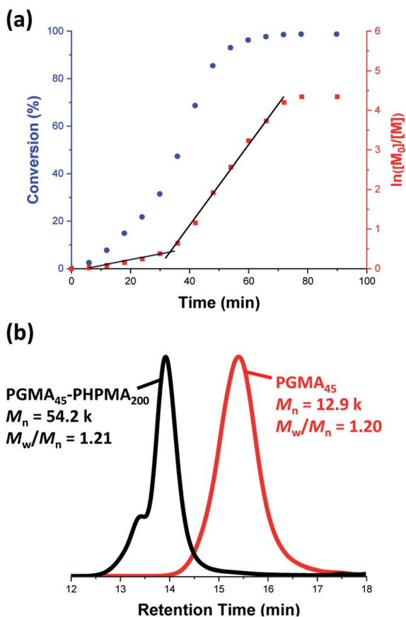
Fig. 3 (a) Kinetic study of the laboratory-based RAFT aqueous dispersion polymerization of HPMA at 70 °C targeting \text{PGMA}_{45} - \text{PHPMA}_{200} diblock copolymer vesicles at 10% w/w solids. The conversion vs. time data and corresponding semilogarithmic plot are denoted by blue circles and red squares, respectively. HPMA conversions were calculated from ^1\text{H} NMR spectra recorded for quenched aliquots of the reaction solution diluted in \text{D}_2\text{O} . (b) DMF gel permeation chromatograms recorded for the final \text{PGMA}_{45} - \text{PHPMA}_{200} diblock copolymer (black curve) prepared via RAFT aqueous dispersion polymerization of HPMA at 70 °C at 10% w/w solids and the corresponding \text{PGMA}_{45} precursor (red curve).
