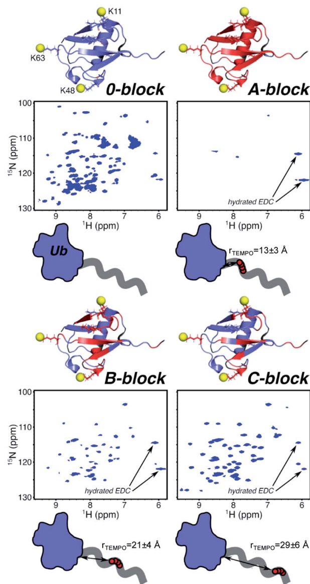
Fig. 2 Structures of Ub (blue) with PRE-broadened residues within conjugates highlighted (red). Reactive amines (yellow spheres) are shown for lysine residues 11, 48, and 63. 1 H/ 15 N-HSQC spectra of each Ub conjugate are shown with annotated peaks resulting from reaction of EDC to form the urea. Schematic representations of conjugates with position of TEMPO (red circles) along the polymer chain (grey line) relative to Ub (blue). Average distances are estimated using Flory–Fox end-to-end distance based on the M_w of the first DMAm block and Mark–Houwink parameters for DMAm in water.
