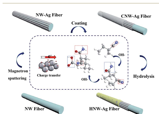
Fig. 2 A schematic representation of the fabricated HNW-Ag.
