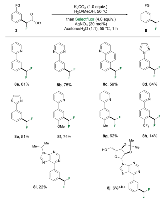
Scheme 3 One pot saponification-fluorodecarboxylation sequence. a Reaction was carried out with the corresponding ethyl acetate and K_2CO_3 (2.0 equiv.) in MeOH/MeOH for saponification, followed by irradiation under 450 nm blue light with (Ir[dF(CF_3)ppy]_2(dtbbpy))PF_6 (6.0 mol%) in DMF (0.1 M) for 24 h at 35 °C. b Traceless removal of acetyl group during saponification. c Conversion determined by LC-MS.
