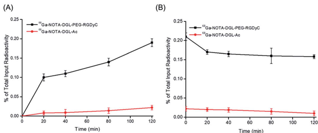
Fig. 5 (A) Radioactivity of ^{68}\text{Ga} in U87 cells incubated with ^{68}\text{Ga} -NOTA-DGL-PEG-RGDyC and ^{68}\text{Ga} -NOTA-DGL-Ac for different times. (B) Elution of ^{68}\text{Ga} -NOTA-DGL-PEG-RGDyC and ^{68}\text{Ga} -NOTA-DGL-Ac in U87 cells.
