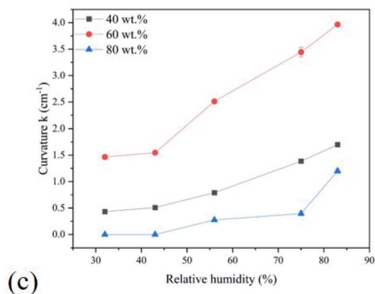
Fig. 4 (a) Digital pictures of curl process of humidity actuators with different MIL-88A loadings (40 wt%, 60 wt% and 80 wt%) at relative humidity variation. (b) Schematic diagram for the calculation of the rotation angle ( \theta ) of the MIL-88A@TPU films (not drawn to scale). (c) Dependent of bending curvature on \Delta RH for the MIL-88A@TPU films with MIL-88A loadings of 40 wt%, 60 wt% and 80 wt% (exposure time was 10 min).
