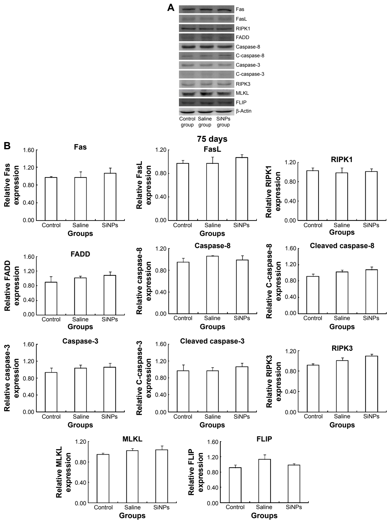
Figure 8 The effects of SiNPs on the expression of proteins in RIPK1 signal pathway at 75 days. Notes: (A) The expression of RIPK1/FADD/caspase-8/cleaved caspase-8/caspase-3/cleaved caspase-3 and RIPK3/MLKL were measured by Western blot assay. (B) Relative densitometric analysis of protein bands were presented. After stopping exposure to SiNPs for 30 days, the effect of SiNPs on the expressions of RIPK1/FADD/caspase-8/cleaved caspase-8/caspase-3/cleaved caspase-3 and RIPK3/MLKL disappeared. Data are expressed as the mean \pm standard error from three independent experiments. The data indicated that the effects of SiNPs on the expression of protein in the RIPK1 signal pathway disappeared after stopping exposure to SiNPs. Abbreviations: SiNPs, silica nanoparticles; FasL, Fas ligand; C-caspase-8, cleaved caspase-8; C-caspase-3, cleaved caspase-3.
