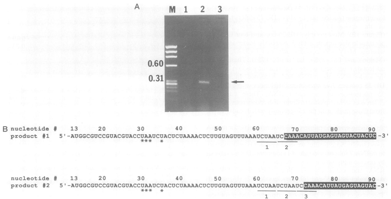
Fig. 4. In vitro transcription of mRNA 6 using exogenous leader RNA. (A) Exogenous leader RNA of 111 nucleotides in length was incubated with mock or MHV-A59 infected cell extracts as described in Figure 2. RNA was extracted and subjected to reverse transcription using oligonucleotide primer #3 specific for mRNA 6 and PCR amplification using primer #2 specific for the exogenous leader sequence. PCR products were analyzed on a 1.5% agarose gel. Lane M: size marker \phi X174 DNA digested with Hae III. PCR products from: mock infected extracts incubated with exogenous leader (lane 1), MHV-A59 infected cell extracts incubated with exogenous leader (lane 2) and MHV-A59 infected cell extract alone (lane 3). (B) Sequence of the mRNA 6 exogenous leader specific PCR product. The 314 nucleotide long PCR product was gel-purified subcloned into pTZ18U and sequenced as described in Materials and methods. The two types of leader/mRNA 6 junction region sequence detected are shown. The DE-25 specific nucleotides are identified by an asterisk, the UCUAA and UCCAA repeats are underlined and the RNA 6 body sequence is highlighted.
