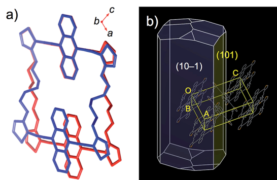
Fig. 6 (a) Superimposed crystal structures of 1c·bent at 20\text{ °C} (HT; red) and -150\text{ °C} (LT; blue). The inserted axes correspond to the geometry at 20\text{ °C} . (b) BFDH morphology calculation of the 1c·bent crystal structure at 20\text{ °C} .
