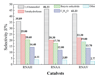
Fig. 13 BED selectivities of the different catalysts. Reaction conditions: 5.0 MPa (pure \text{H}_2 ), 393 K, 0.5 g catalyst, 30 mL 1,4-butenediol (35 wt% in water).
