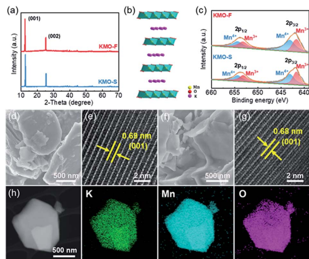
Fig. 3 Structure characterization of KMO-F and KMO-S. (a) XRD patterns of KMO-F and KMO-S. (b) Simulated crystal structure of layered K_xMnO_2 . (c) XPS spectra of KMO-S and KMO-F. SEM image of (d) KMO-F and (f) KMO-S. HRTEM images of (e) KMO-F and (g) KMO-S. (h) STEM image of KMO-F with corresponding elemental mappings of K , Mn , and O .
