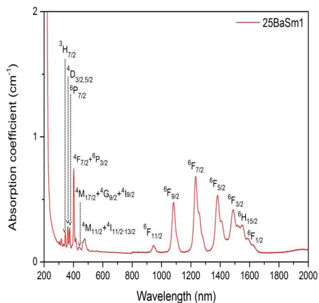
Fig. 4 The absorption spectra of series B glasses for (a) all concentrations and (b) 25 mol% of BaO and 1 mol% of \text{Sm}_2\text{O}_3 .
