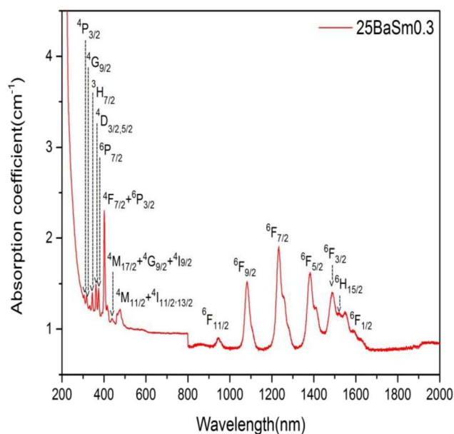
Fig. 3 The absorption spectra of series A glasses for (a) all concentrations and (b) 25 mol% of BaO and 0.3 mol% of \text{Sm}_2\text{O}_3 .
