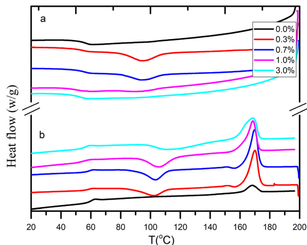
Fig. 5 DSC thermograms of PLLA and PLLA-BDOBH at (a) a cooling rate of 10\text{ }^{\circ}\text{C min}^{-1} from 190; (b) a heating rate of 10\text{ }^{\circ}\text{C min}^{-1} from 20\text{ }^{\circ}\text{C} .
