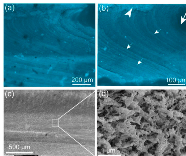
Fig. 2. (a) Confocal microscope image showing distribution of polysaccharide-based biopolymers within the growth bands stained with Calcofluor White M2R (b) Higher magnification of inner portion of the outer shell layer. The white arrowhead points towards outer portion of the outer shell layer. The white arrow defines the outside surface of the shell. (c, d) Field emission gun scanning electron micrographs of the shell after etching showing ultrastructures and organic fibres. Higher magnification reveals rod-type crossed lamellar parallel to the co-marginal plane.
