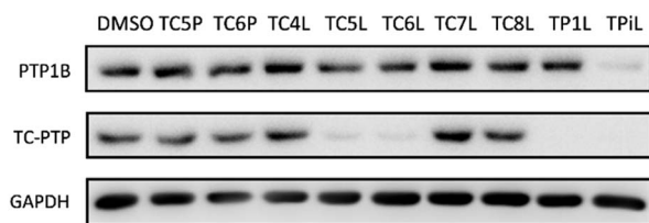
Fig. 2 Degradation assay results of second-generation TC-PTP PROTACs. HEK293 cells were treated with DMSO or 1 \mu\text{M} indicated compounds for 16 hours.
