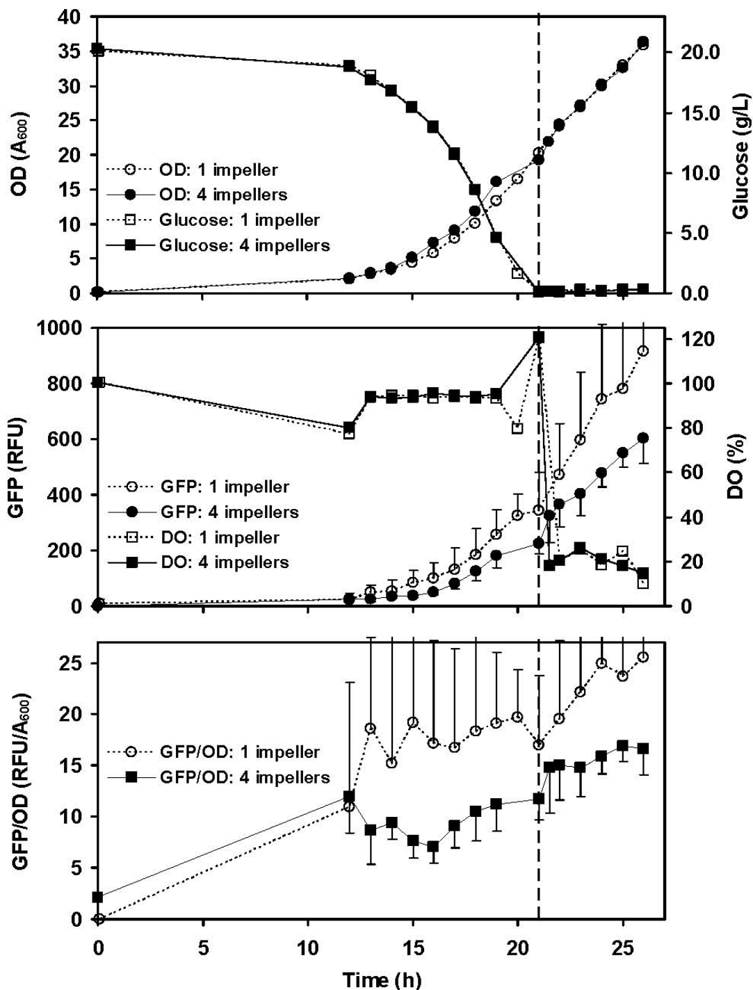
Figure 3 Growth and GFP expression during fed batch fermentations with either one or four impellers (all else equal). (A) Biomass, measured as optical density (OD, A_{600} ), and glucose concentration (g/L), (B) Green fluorescent protein expression (RFU) and dissolved oxygen concentration (% air saturation) and (C) specific GFP expression (RFU/ A_{600} ). Dashed vertical line at 21 hours shows where batch phase ended and feeding began. Error bars represent standard deviation, drawn in only one direction for clarity.
