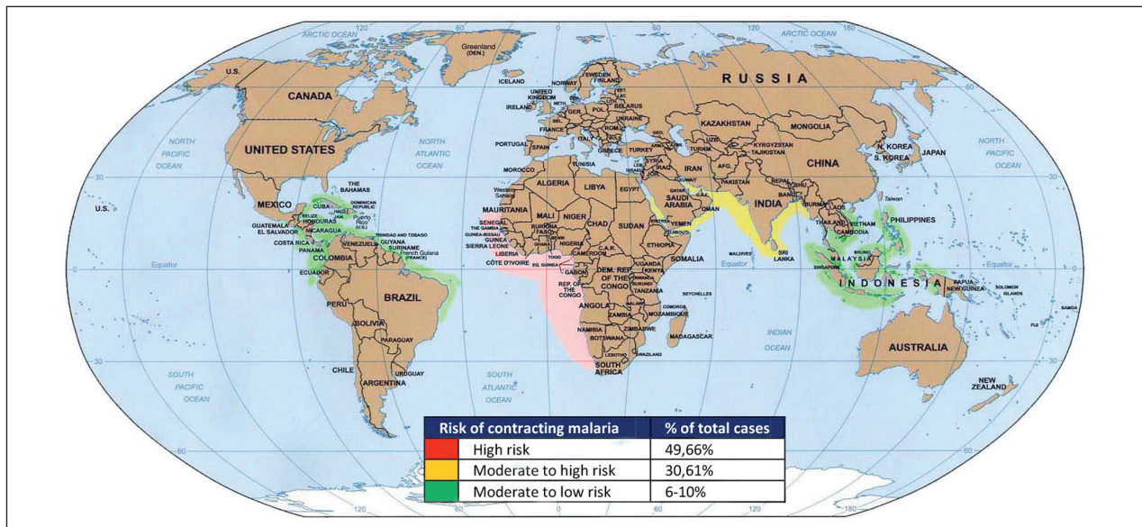
Figure 2. Geographic areas at risk of malaria infection for seafarers (based on the number of reported malaria cases)
