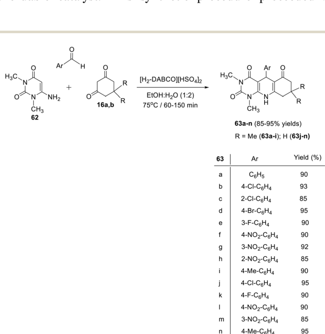
Scheme 35 Synthesis of pyrimido[4,5- b ]quinolines 63a–n utilizing [H 2 -DABCO][HSO 4 ] 2 as the catalyst.
