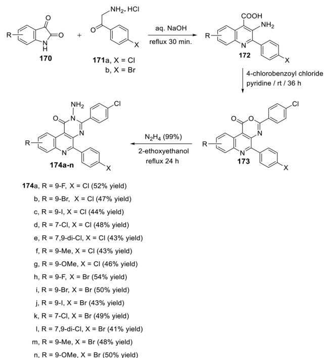
Scheme 73 Synthesis of new 2-amino-pyrimido[4,5-c]quinolin-1(2H)-ones 174a–n .
