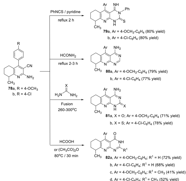
Scheme 44 Synthesis of some new derivatives of tetrahydropyrimido[4,5- b ]quinolines 79–82.
