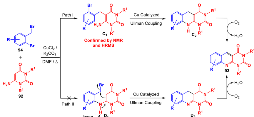
Scheme 53 Proposed mechanism for the formation of 93 from 92 and 94 under reflux conditions.
