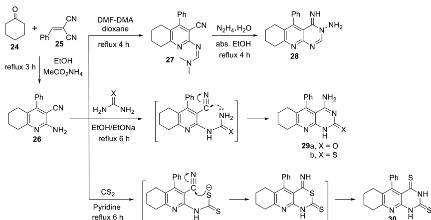
Scheme 10 Facile synthesis of new 6,7,8,9-tetrahydropyrimido[4,5- b ]quinolines 28–30.
