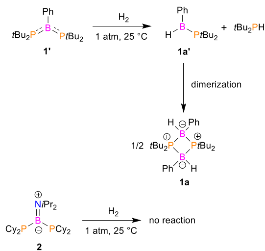
Scheme 1. Reactions of 1 and 2 with Dihydrogen
