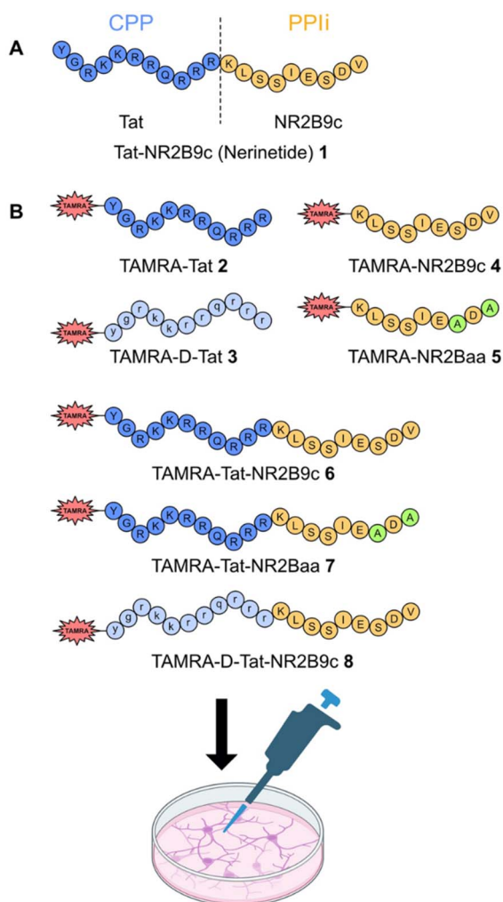
Fig. 1 Overview of peptides used in this study. (A) Structure of nerinetide (1) and (B) TAMRA labelled analogues of nerinetide (6), nerinetide fragments (2, 4) D-Tat (3), D-Tat-NR2B9c (8), and inactive nerinetide PPIi (5, 7).
