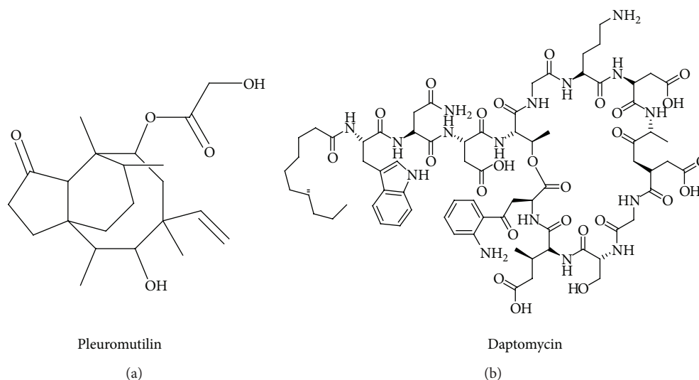
FIGURE 1: Chemical structures of pleuromutilin and daptomycin.
