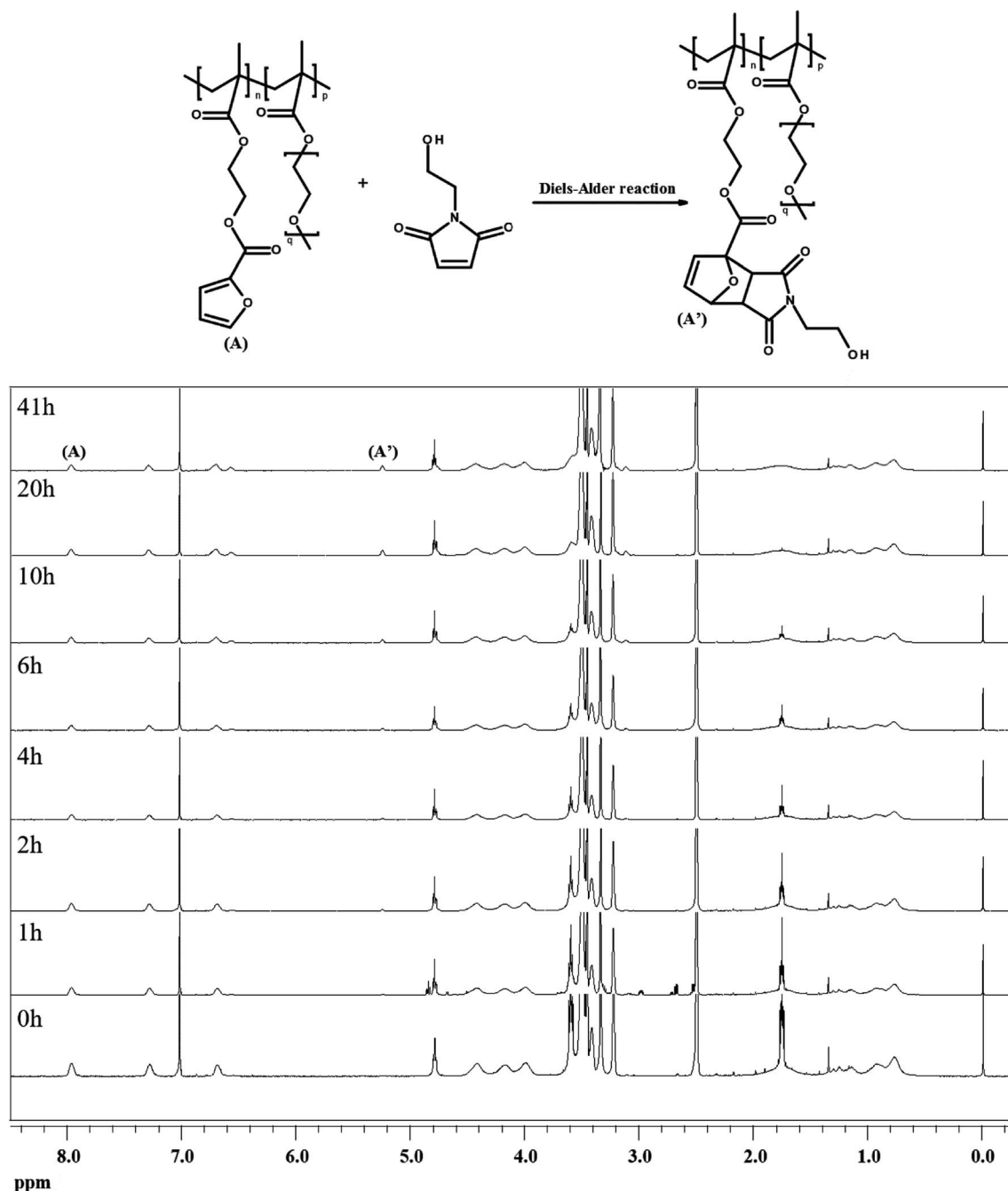
Fig. 6 ^1\text{H-NMR} spectra of the mixture of dPFMA64 and mM kept at 60\text{ }^\circ\text{C} for 0 to 41 h.
