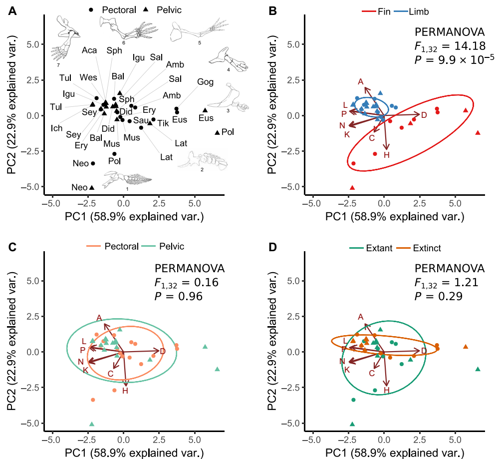
Fig. 2. Biplots of the first two PCA components of topological variables for pectoral (circles) and pelvic (triangles) appendages combined. (A) Distribution of pectoral and pelvic appendages for each taxon in the sample (abbreviated by the first three letters of the genera). For reference, we included line drawings representing different appendages: (i) Neoceratodus pectoral, (ii) Latimeria pelvic, (iii) Eusthenopteron pelvic, (iv) Gogonasmus pectoral, (v) Salamandra pectoral, (vi) Acanthostega pelvic, and (vii) Sphenodon pectoral. (B) Comparison of limbs versus fins (i.e., appendages with and without digits, respectively) showed that they occupy different regions of the morphospace. (C) Comparison of pectoral versus pelvic appendages showed that they occupy overlapping regions of the morphospace. (D) Comparison of extant versus extinct taxa showed that they occupy the PC2 axis in different ways. Red arrows show the contribution to the first two PCA components of each network variable: (N) nodes, (K) links, (D) density, (C) clustering coefficient, (L) path length, (H) heterogeneity, (A) assortativity, and (P) parcellation.
