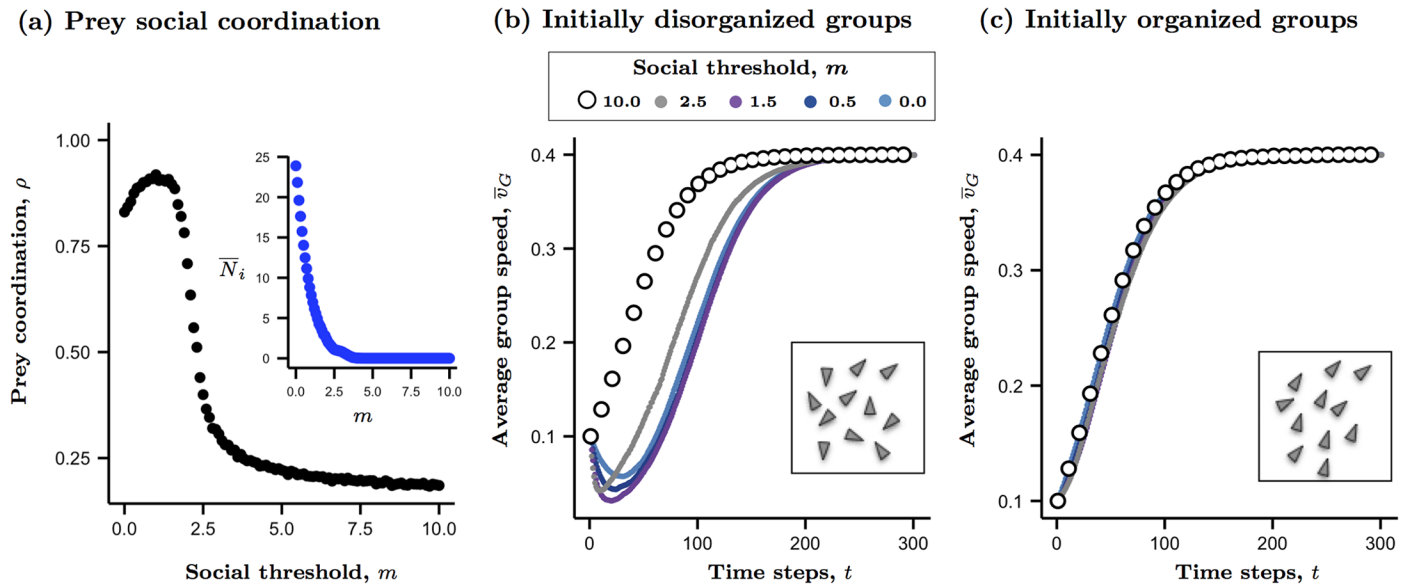
Fig 1. The influence of individual social thresholds and initial group organization on attention levels, collective coordination, and average individual speed. As the individual’s social threshold increases ( m ), overall coordination in the group begins to rise then decays rapidly (a) because individual’s are less likely to pay attention to their neighbors (a, inset). Over time, the group’s average speed is a function of both the individual-level interactions and the initial conditions (b, c). Increases in social thresholds range from asocial behavior (random walk; black open circles) to social interactions of varying degrees (colored points). Insets in (b) and (c) illustrate the initial orientations of the prey. Increased social attention is reflected by a larger number of influential neighbors, N_i = |\mathbf{N}_i| (Eq 4). When groups are initially disorganized (b) a lag in the average individual’s departure speed emerges as a consequence of the time needed to come to a directional consensus. When groups are already organized their social interactions have little feedback on collective speed (c). Model parameters: group size = 25, m : {0, 1.5, 2.5, 10.0}, v^* = 0.44 . Data represent mean values of 1,000 replicates per setting. Additional parameters are provided in S1 Table .
