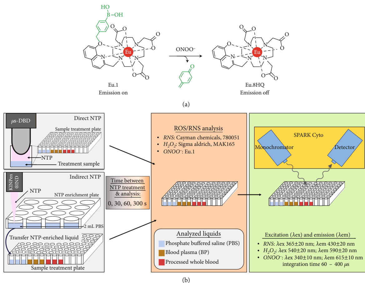
FIGURE 1: Experimental design to determine the stability of persistent ROS/RNS. (a) The mode of action of Eu.1 for detecting ONOO - is shown. (b) PBS (blue), BP (yellow), and processed whole blood (red) were analyzed following direct and indirect NTP treatment. Following treatment, the sample was either analyzed immediately (0 s) or after a delay (between 30 and 300 s) for RNS, H 2 O 2 , or ONOO - ( \mu s-DBD: microsecond-pulsed dielectric barrier discharge; \lambda_{ex} : excitation wavelength; \lambda_{em} : emission wavelength).
