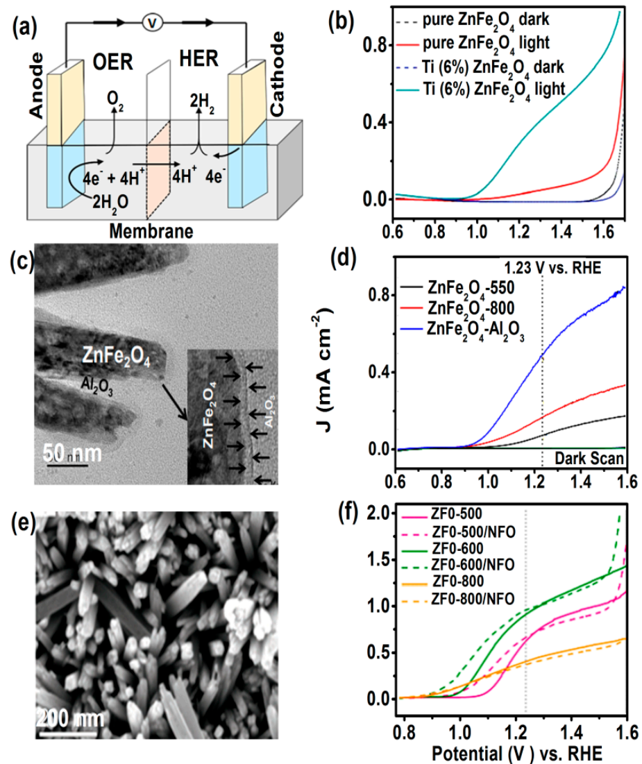
Figure 15. (a) Schematic of electrolysis cell for water splitting, (b) current density J vs. potential curves, V of \text{ZnFe}_2\text{O}_4 photoanodes (Reproduced with permission from [92]. Copyright Royal Society of Chemistry, 2017). (c,d) TEM image of \text{ZnFe}_2\text{O}_4\text{-Al}_2\text{O}_3 and corresponding J vs. V curves (Reproduced with permission from [93]. Copyright Royal Society of Chemistry, 2018). (e) SEM images \text{ZnFe}_2\text{O}_4 nanorod, ZFO-500 (f) J vs. V curves (Reproduced with permission from [95]. Copyright Wiley, 2018).
