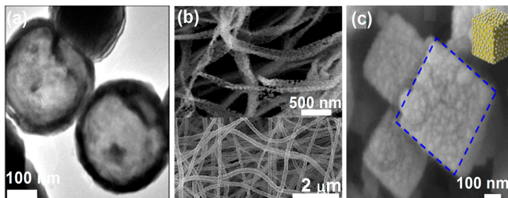
Figure 9. (a) High-resolution TEM of Zn_{0.3}Fe_{2.7}O_4 nanospheres (Reproduced with permission from [52]. Copyright American Physical Society, 2019). (b) SEM images of nanotubes in the lower panel and SEM images of nanobelt in the upper panel (Reproduced with permission from [58]. Copyright Elsevier, 2018). (c) SEM images of hollow porous core-shell ZnFe_2O_4/AgCl nanocube (blue dotted line represents cubic facet) coated with EDTA-Ag nanoparticles (Reproduced with permission from [59]. Copyright Elsevier, 2020).
