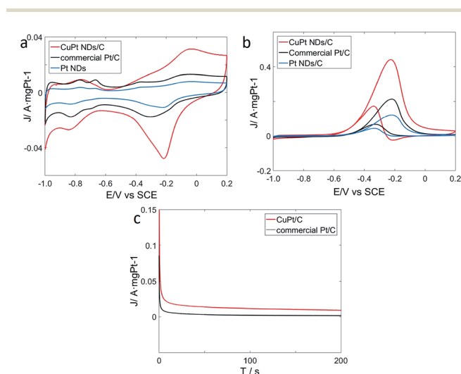
Fig. 8 (a) Cyclic voltammetry (CV) curves of the catalysts in 0.5 M NaOH, (b) CV curves of the catalysts in 0.5 M NaOH and 0.5 M \text{CH}_3\text{OH} , (c) current–time ( i – t ) curves of the catalysts in 0.5 M NaOH and 0.5 \text{CH}_3\text{OH} at -0.32 \text{ V} .
