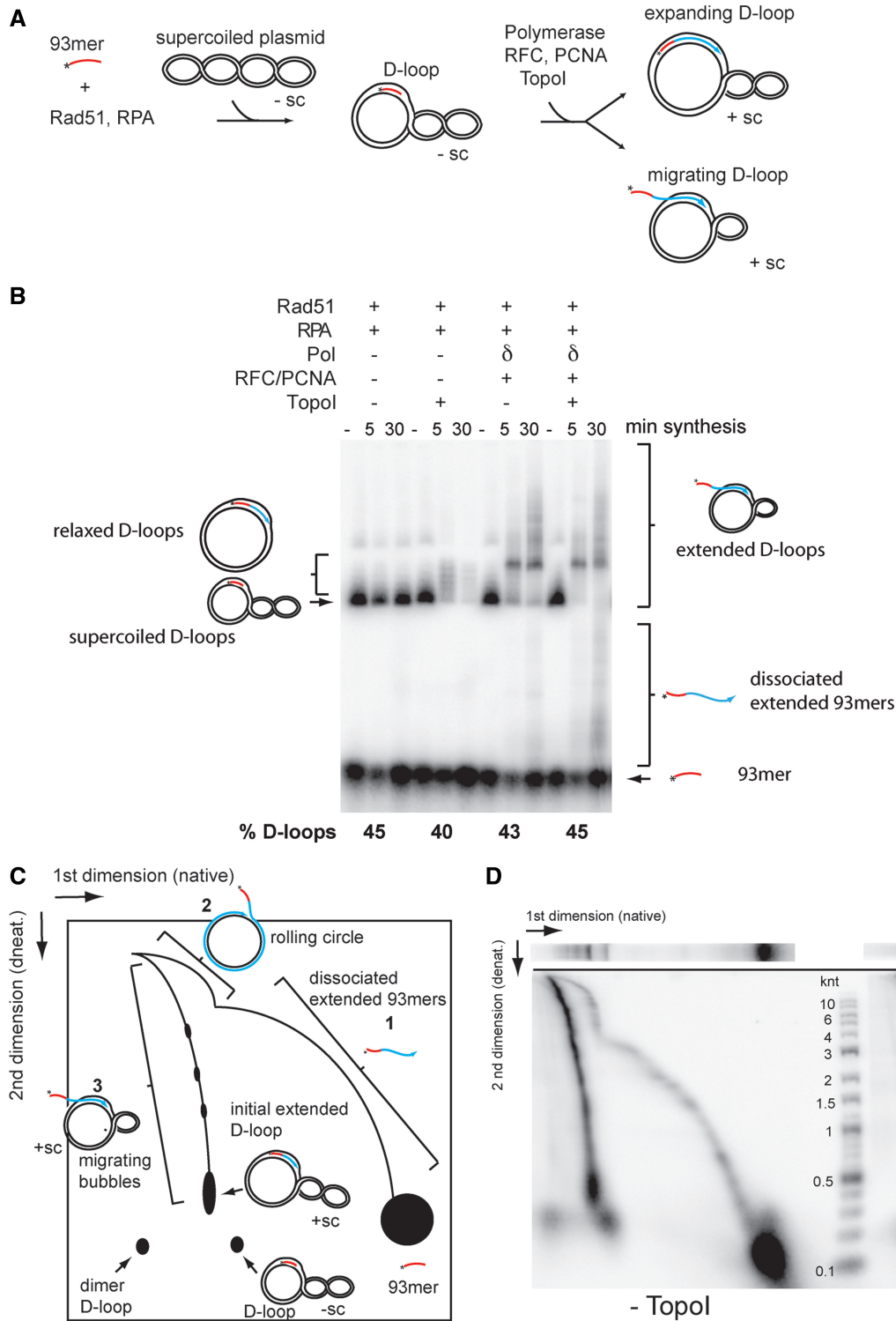
Figure 4. DNA synthesis proceeds via a migrating D-loop. (A) Experimental scheme. Single-stranded 93mer is 32 P-end-labeled (asterisk). The dsDNA substrate contains ~15 negative supercoils (-sc). On D-loop formation with the 93mer, this changes to ~6 negative supercoils. For each 10.5 nt synthesized, one positive supercoil (+sc) is added, resulting in the accumulation of positive supercoils during D-loop extension. (B) Analysis of D-loop formation and DNA synthesis in the presence or absence of TopoI as measured by 0.8 % native agarose gel electrophoresis. (C) Cartoon depicting analysis of products by two-dimensional gel electrophoresis. (D) Two-dimensional gel electrophoresis of D-loops extended by Pol δ in the presence or absence of TopoI.
