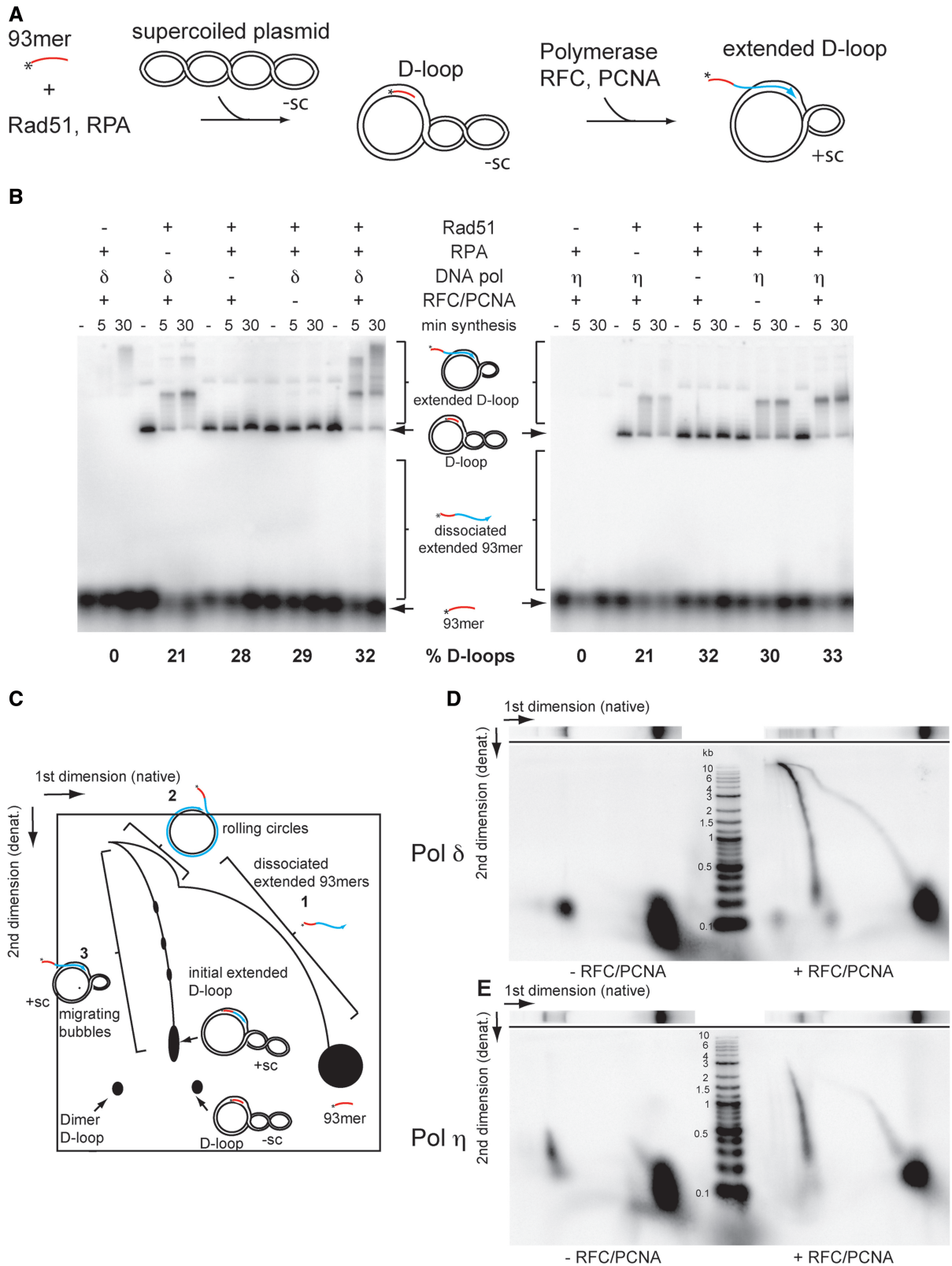
Figure 2. D-loop formation and DNA synthesis. (A) Experimental scheme. The single-stranded 93mer is 32 P-end-labeled (asterisk). See also Figure 4A legend for aspects of topology. (B) Analysis of D-loop formation and DNA synthesis by Pol \delta and Pol \eta at D-loops as measured by 0.8 % native agarose gel. Percent D-loops were determined at 0 min. (C) Cartoon depicting analysis of products by two-dimensional gel electrophoresis. (D) Two-dimensional gel electrophoresis of D-loop reactions extended by Pol \delta in the presence or absence of RFC, PCNA after 30 min extension time. (E) Same as in D, using Pol \eta .
