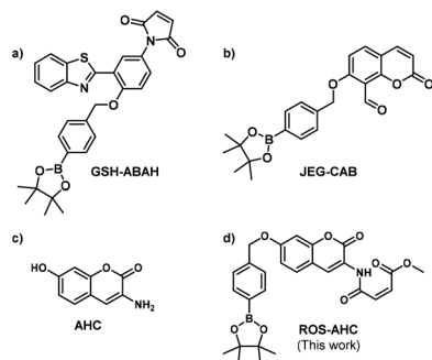
Fig. 1 (a) GSH-ABAH, previously reported probe for simultaneous detection of \text{ONOO}^- and GSH. (b) JEG-CAB, previously reported probe for simultaneous detection of \text{ONOO}^- and GSH. (c) AHC – a core fluorescent unit that enables the synthesis of ‘AND’ based fluorescent probe for the detection of \text{ONOO}^- and GSH (d) ROS-AHC, a novel probe detailed in this work for simultaneous detection of \text{ONOO}^- and GSH.
