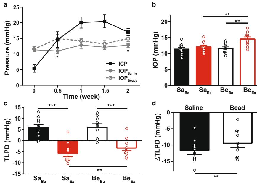
Fig. 2 Changes in IOP, ICP, and TLPD. a Combined plot of mean baseline (time = 0) and experimental (all other time points) IOP and ICP values. ICP, IOP elevation (IOP Beads ; gray open circle connected with dotted line) and contralateral control (IOP Saline ; gray solid circle connected with a solid line) are shown. b Mean baseline IOP (black bars; Sa Ba = saline baseline; Be Ba = beads baseline) and mean experimental IOP (average of all post-injection values, per eye; red bars; Sa Ex = saline experimental; Be Ex = beads experimental). c Mean baseline and experimental values for TLPD. Baseline TLPDs are in black and experimental TLPDs are in red. Experimental values of TLPD are different from baseline values (Sa Ba vs Sa Ex and Be Ba vs Be Ex ; both <0.001). d \Delta TLPD for saline- and bead-injected animals. \Delta TLPD represents the change in TLPD from baseline (experimental – baseline). For all panels, N = 10 and error bars = 1 SEM. * p < 0.05 , ** p < 0.01 , *** p < 0.001 .
