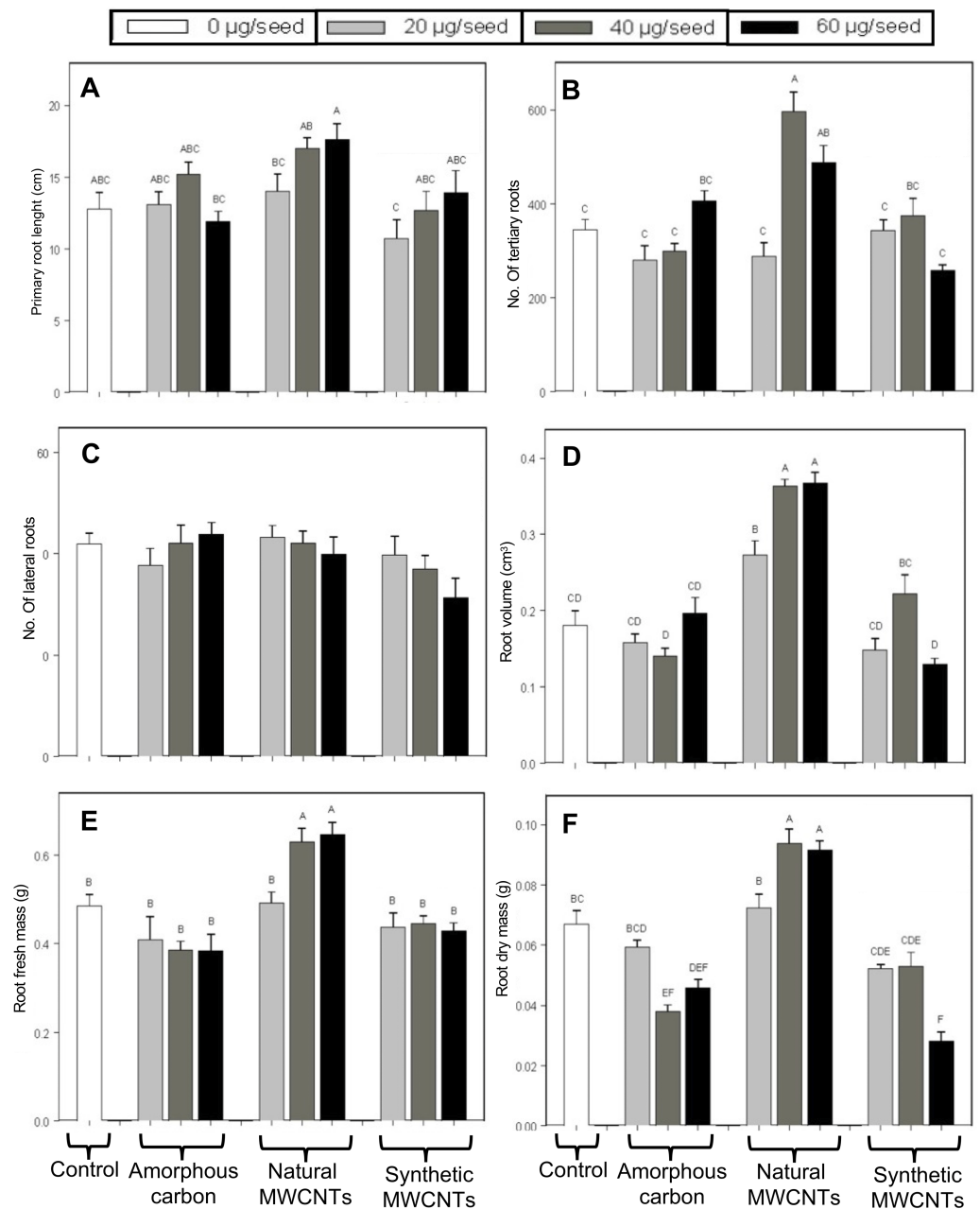
Figure 4 Effect of synthetic MWCNTs, amorphous carbon and natural MWCNTs on root architecture of Eysenhardtia polystachya plants. Seeds of E. polystachya were supplemented with 1.0 mL suspension containing either 0 (control), 20, 40, or 60 µg/mL of the different carbon materials. After 60 days of planting the plants were harvested and root architecture variables were recorded. (A) Primary root length, (B) lateral roots number, (C) tertiary roots number, (D) root volume, (E) root fresh weight, and (F) root dry weight. Bars represent mean \pm SE of three independent assays. n = 8 . One-way analysis of variance (ANOVA) was carried out with Tukey's post hoc test; statistical significance ( P < 0.05 ) between treatments with respect to control is indicated with different lowercase letters.
