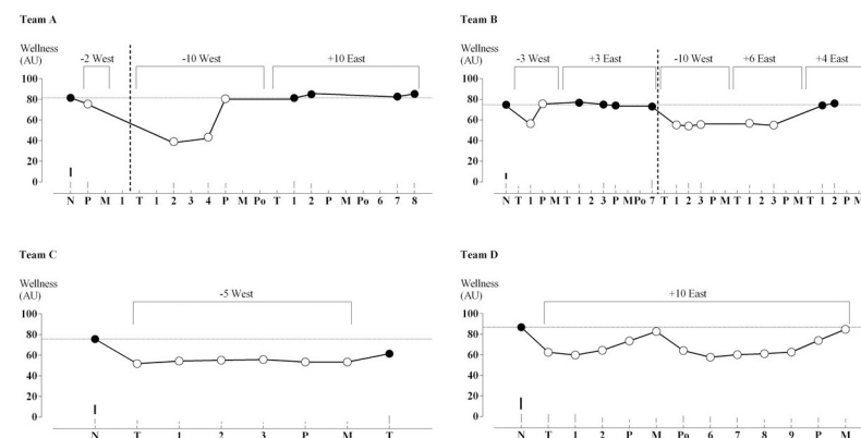
Fig 2. Estimated wellness after adjusting for peri-match effects during days spent overseas and upon return compared to normal days. Thin lines are within players SD for each day. Thick lines are observed between players SD for each team. Dotted horizontal lines are normal wellness scores for each team. Dashed vertical lines represent a time gap occurred during data collection. Square brackets report number of time zones crossed and direction of travel. Black symbols are home days, empty symbols are overseas days. X-axis abbreviations: N, normal nights; P, pre-match nights; M, match nights; Po, post-match nights; T, travel nights; numbers represent days following travel.
