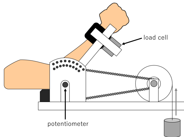
Figure 1 Experimental setup for maximal isometric (MVC) and dynamic contraction tasks. Schematic diagram of the experimental set up for conducting the maximal isometric (MVC) and dynamic contraction tasks. The participants sat on a chair adjusted for the testing position. Their right arms were fixed to the dynamometer with the shoulder flexed at 90° and the forearm in a neutral position.
