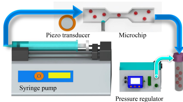
FIG. 1. The microfluidic chip and its associated flow control system. The 20 mm microchannel showcases a rectangular cross section ( H = 150\ \mu\text{m} \times W = 450\ \mu\text{m} ), transitioning to a smaller square cross section ( H = 150\ \mu\text{m} \times W = 150\ \mu\text{m} ) through a linear narrowing with a 45^\circ angle, forming a two-dimensional nozzle converging toward the constriction. At the nozzle's onset, there is a cavity with a width of w = 80\ \mu\text{m} and a length of h = 500\ \mu\text{m} . The microbubble is stimulated by a piezoelectric transducer, while the syringe pump regulates the flow rate, and a pressure regulator maintains liquid and bubble pressure for size stabilization.
