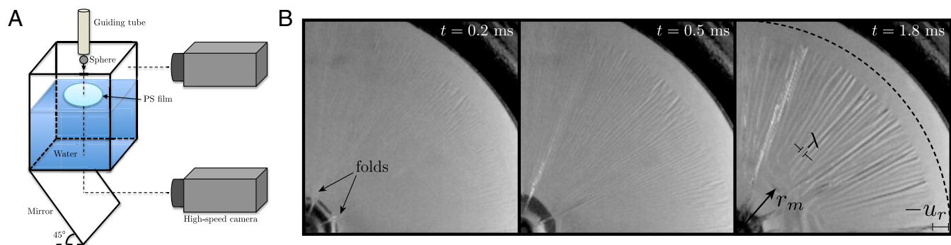
Fig. 2. (A) Schematic of the experimental setup used to drop steel spheres onto floating PS sheets. (B) Time series of 1 quadrant of a sheet ( h = 450 nm, R_f = 17.40 mm) impacted by a sphere (radius R_s = 1.75 mm, V = 1.17 ms ^{-1} ) and imaged from below. Note that wrinkles coarsen during the experiment, trebling their mean wavelength in \sim 1.5 ms. Also highlighted in the images are the onset of folds, the propagation of a transverse wave (visible at radius r_m ), and the retraction of the sheet edge (the initial position of which is shown as the dashed circle).
