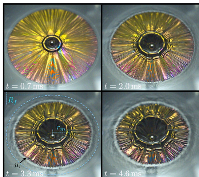
Fig. 1. A steel sphere (radius R_s = 1.25 \text{ mm} ) impacts a PS sheet (thickness h = 350 \text{ nm} , radius R_f = 17.15 \text{ mm} , floating at a water to air interface) at speed V = 0.72 \text{ ms}^{-1} . Impact draws the outer edge of the sheet inward by a distance -u_r(R_f, t) , compressing the sheet even in regions where it remains flat [beyond the propagating transverse wave at r = r_m(t) ]. The number of radial wrinkles in the sheet decreases with time (i.e., with increasing impact depth Vt ), in contrast to the static indentation of a floating sheet (15, 19).
