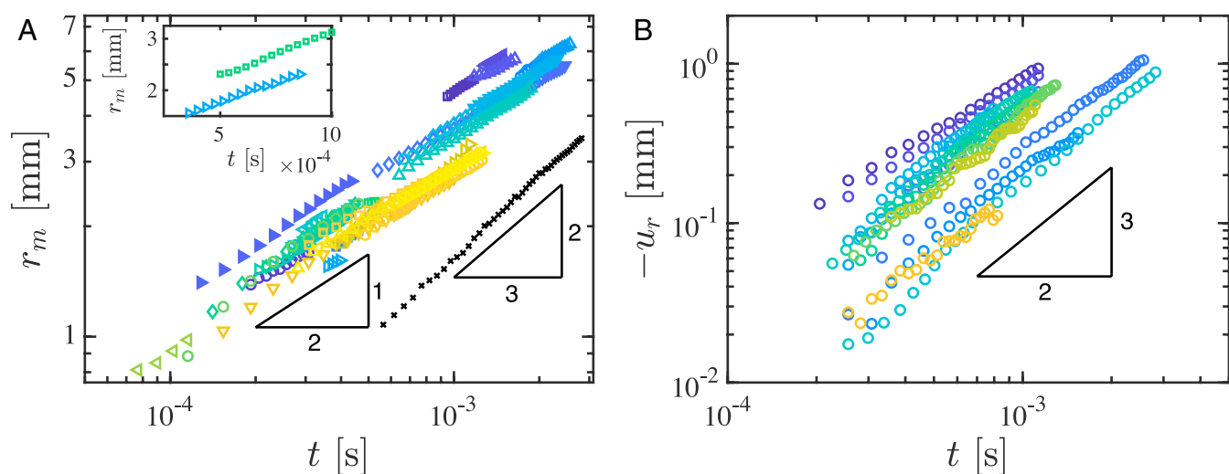
Fig. 3. The propagation of the transverse wave and subsequent retraction of the sheet edge. (A) Measurements of the radial position of the capillary wave front on a liquid-to-air interface with no elastic sheet ( \times ) give r_m \propto t^{2/3} , different from the behavior with that for an ultrathin PS sheet (colored points). (Inset) Wave propagation depends on R_f ( \approx 5.51 mm for \triangleright and 13.30 mm for \square ). (B) The sheet's edge moves radially inward by an amount -u_r(R_f) \propto t^{3/2} , corresponding to negligible radial stretching. (Experimental parameters for the data in A and B are given in SI Appendix, Tables S1 and S2, respectively.)
