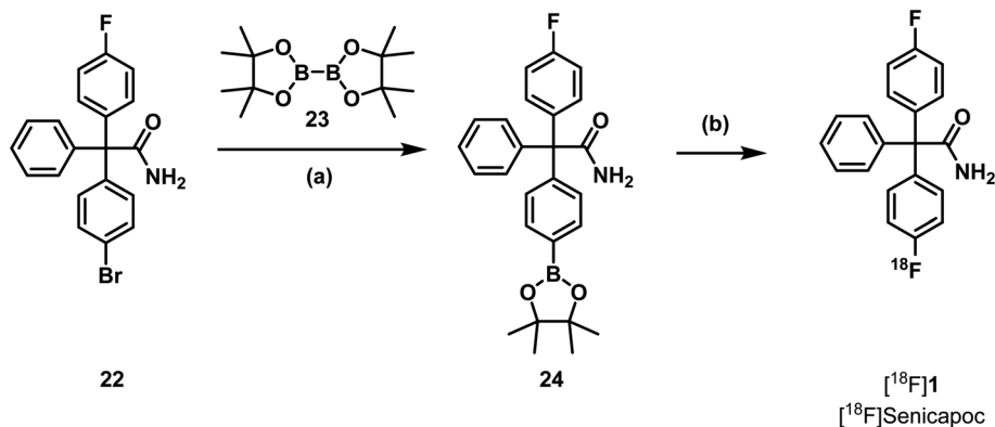
Scheme 6 Last step of the synthesis of the pinacol boronic ester 24 and radiosynthesis of [^{18}\text{F}]\text{senicapoc} ( [^{18}\text{F}]\mathbf{1} ). Reagents and reaction conditions: (a) \text{Pd}(\text{dppf})\text{Cl}_2 , KOAc, dioxane, RT- 50 °C, 5 h, 15%. (b) cartridge: Sep-Pak® Light QMA Fa. Waters®, [^{18}\text{F}]\text{TTEAF} , butan-1-ol, \text{Cu}(\text{OTf})_2\text{py}_4 , DMF, 110 °C, 10 min, 0%.
