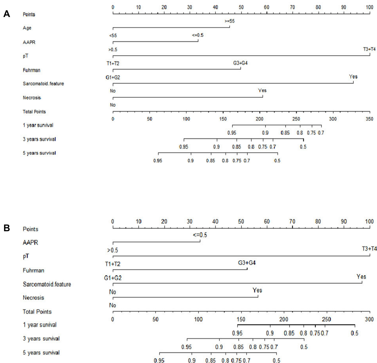
Figure 4 Nomogram for predicting (A) OS and (B) CSS in non-metastatic RCC patients.
