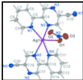
Fig. 1. The atom-numbering scheme of the title compound. Displacement ellipsoids are drawn at the 30% probability level.
