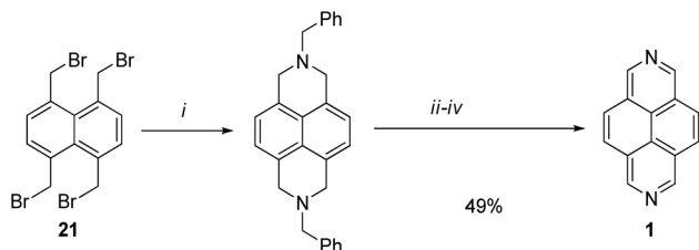
Scheme 8 Synthesis of 2,7-diazapyrene from 1,4,5,8-tetrakis-(bromomethyl)naphthalene. Reagents and conditions: (i), PhCH 2 NH 2 , K 2 CO 3 ; (ii), ClCO 2 Et, THF, 55 °C; (iii), KOH, H 2 O-1,4-dioxane = 1 : 1; (iv), MnO 2 , Benzene, reflux.
