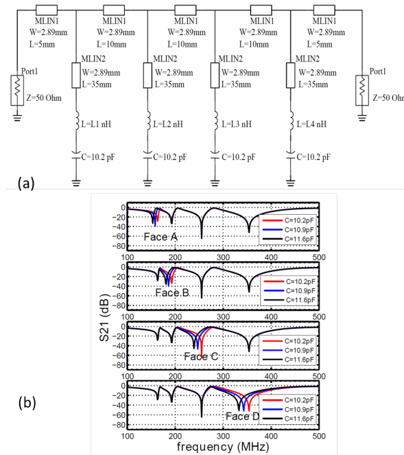
Figure 3. (a) The schematic of the circuit simulation. C_1 = 10.2 pF; L_i ( i = 1, 2, 3, 4 ) is 82 nH, 56 nH, 27 nH and 8.2 nH, respectively. (b) Transmission spectrum given by circuit simulations. The four sub-figures indicate the change in capacitance at four sensing elements, A, B, C, D, with different inductance values. In each sub-figure, curves with different colors represent different capacitance values.
