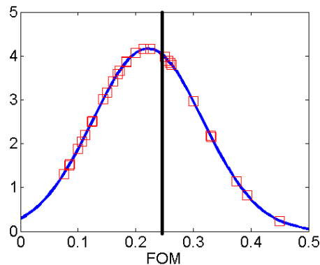
Figure 7. The comparison of the sensor figure-of-merit (FOM) with commercial sensors. All data points are fitted in a Gaussian distribution, with mean 0.221 and a standard deviation of 0.096. Squares are FOM from commercial sensors, and the black line indicates the FOM of the designed sensor.
