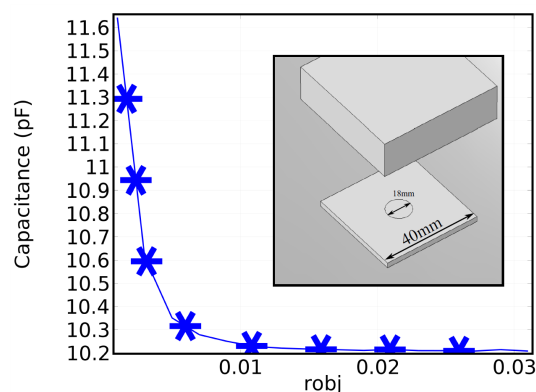
Figure 2. Simulation of the patch sensor and its capacitance change with the distance of an object. The patch has a radius of 9 mm, on FR4 substrate of a size of 40 mm × 40 mm and a thickness of 1.2 mm. Simulations are done in commercial software COMSOL Multiphysics.
