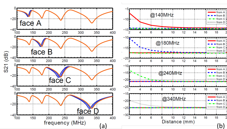
Figure 6. (a) Measured transmission spectrum. The four sub-figures indicate the change in capacitance at four sensing elements with different inductance values. In each sub-figure, curves with different colors represent different distances between the target and sensing element; (b) The four sub-figures are for the S_{21} at different frequencies. The four curves in each sub-figure represent the object coming from four different directions.
