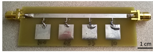
Figure 9. Fabricated capacitive sensor array on a microstrip line with connected surface mount inductors.
