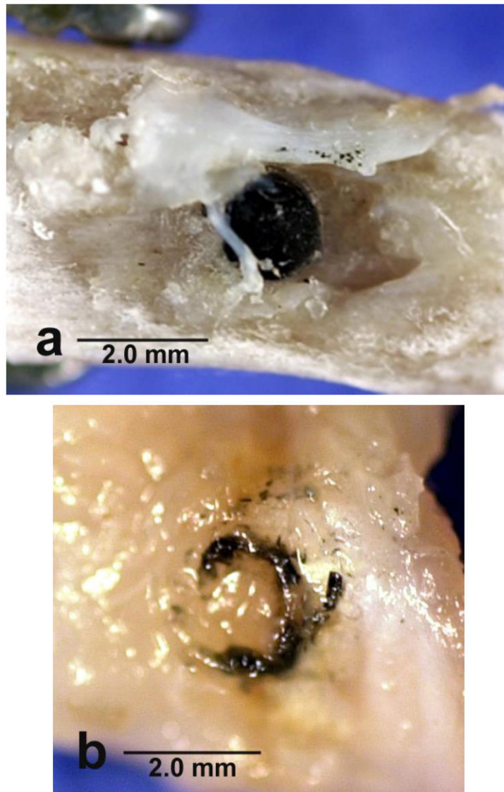
Figure 9. Photographs (a) implant extends above cortical bone with exuberant osteoid production stimulated from small carbon fiber fragments extruded out of the marrow space; (b) dissected soft tissue overlying the cortical bone integrated with carbon fiber fragments from the end of the implant.
