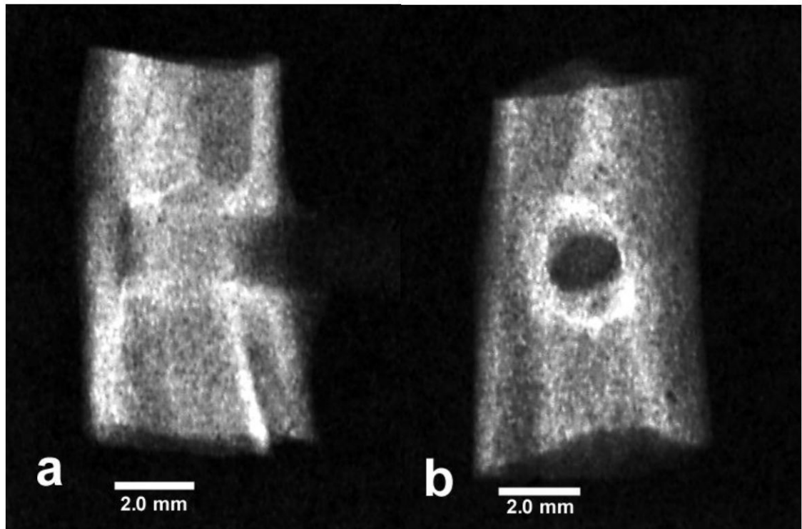
Figure 6. X-rays epoxy/carbon fiber PMC (a) Lateral view (b) Frontal view.
