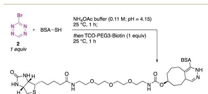
Scheme 6 Labelling of BSA. One-pot procedure for the functionalisation of BSA with 3-Br-Tet ( 2 ) and subsequent iEDDA with TCO-PEG3-biotin.
